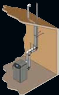
Direct-Vent Vertical
