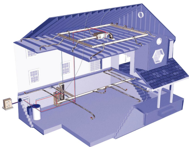
Typical ductwork layouts showing 2 Unico systems —one located in the attic and one located in the basement.
